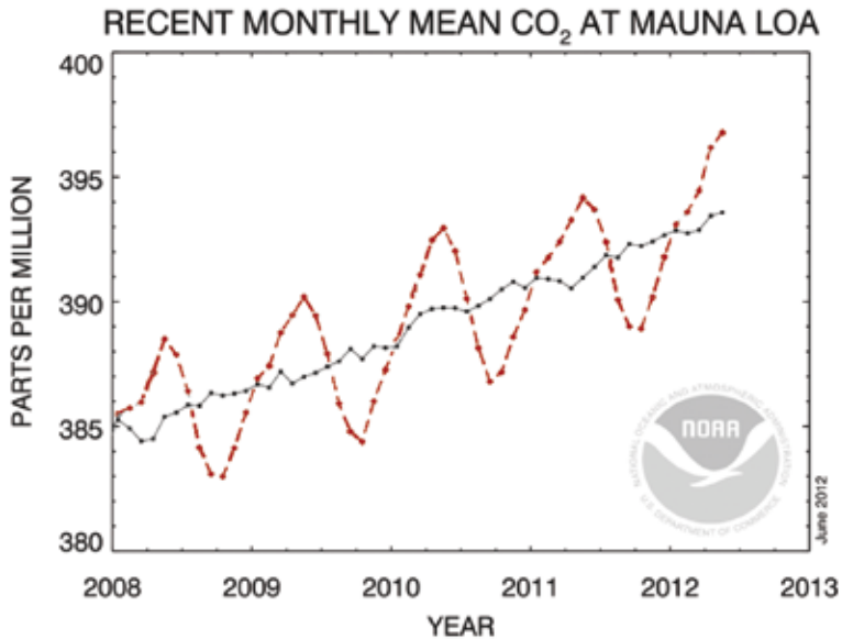
Figure 1.4: Seasonal fluctuation in atmospheric carbon dioxide (CO 2 ) at the Mauna Loa Observatory since 2008. The black line shows the overall trend. The red line shows carbon levels month by month. Carbon levels drop during the northern summer because plants absorb more carbon in the growing season and there is much more land for plants to grow on in the north than in the south. Source: National Oceanic and Atmospheric Administration (NOAA).
